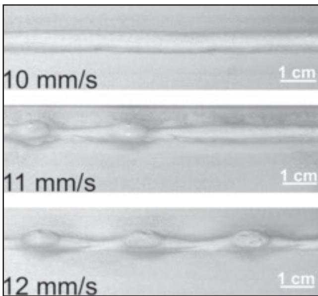
Fig. 6 — Top view of GMA welds produced using 6.3 kW welding power, argon shielding gas, and at various welding speeds.
