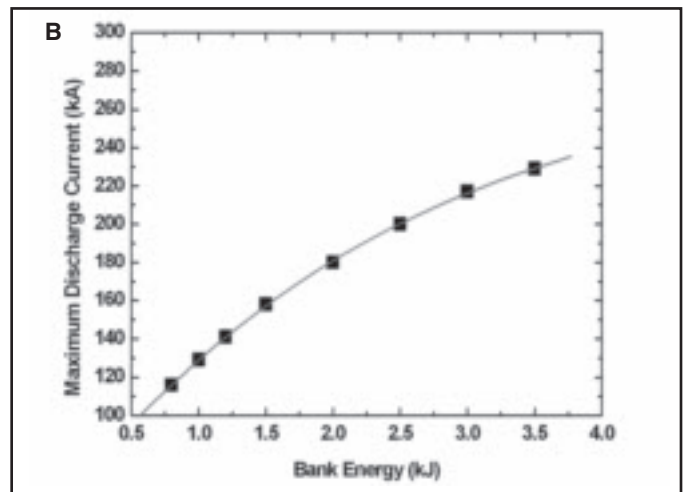
Fig. 6 — A — Typical current signal at 1.4-kJ discharge (200 µF/3.8 kV); B — bank energy vs. maximum discharge current.
