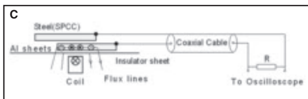
Fig. 3 — General outlines of apparatus. A — Cross-section view of the coil containing lap of Al/steel (SPCC) sheets and discharge circuit; B — plan view of coil with discharge circuit; C — collision speed measurement. C denotes the capacitor bank and G the gap switch.
