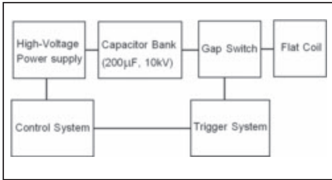
Fig. 4 — The block diagram of the discharge system.
