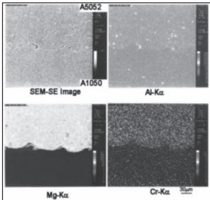
Fig. 11 — SEM-SE image and EPMA result for Al, Mg, and Cr distribution for A1050/A5052 sample.
