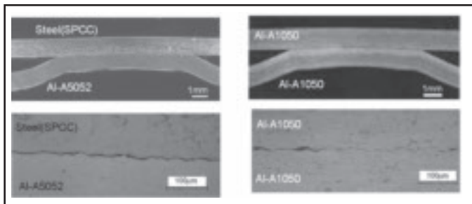
Fig. 8 — Typical microstructure of joined interface zone for A1050/A1050 and A5052/SPCC.
