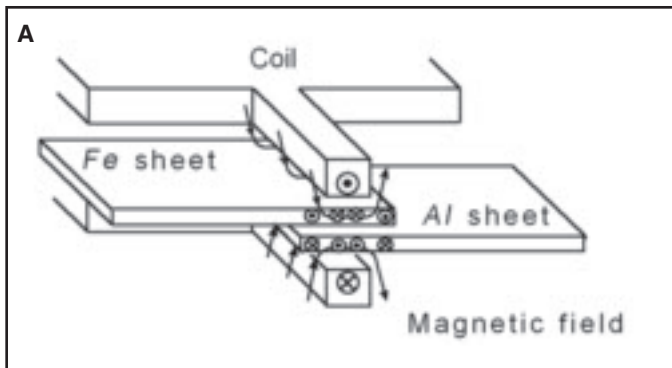
Fig. 1 — MPW coil structure. A — Double-layer, H-shaped flat coil; B — one-layer E-shaped flat coil.
