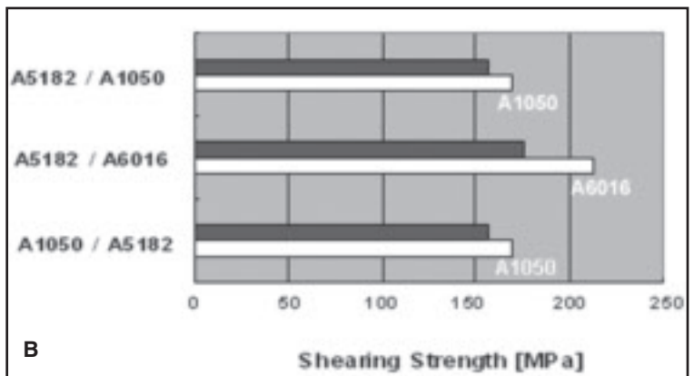
Fig. 15 — Comparison of the maximum tensile shear strength for the following: A — The same aluminum alloy combinations; B — different aluminum alloy combinations: ■ The maximum tensile shearing strength of welded sample. □ The maximum tensile shearing strength of the base alloy without weld.
