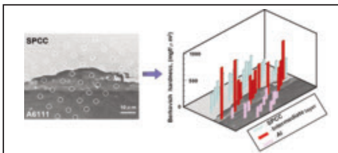
Fig. 12 — Typical microstructure of the interface layer of the A6111/SPCC sample, including Berkovich hardness indentation across the interface.
