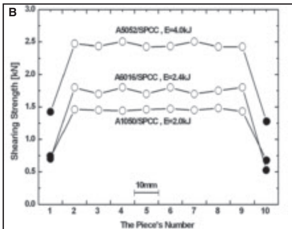
Fig. 13 — Distribution of tensile shear strength for ten divided pieces of the welded samples. A — A1050/A1050, A3004/A3004, and A5182/A5182 sheets; B — A1050/SPCC, A5052/SPCC, and A6016/SPCC sheets: ○ The rupture of base metal, ● the rupture of the welded area.
