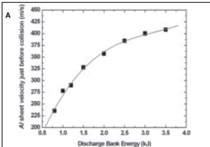
Fig. 7 — The speed of the Al sheet just before collision vs. the following: A — Discharge bank energy; B — maximum discharge current.
