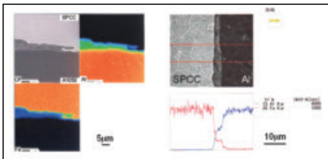
Fig. 10 — EPMA result for Fe and Al distribution across the SPCC/A1050 interface layer.
