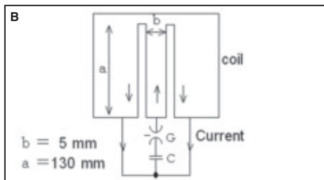
Fig. 2 — Principle of MPW for welding of the Al/steel sheet sample (cross-section view).
