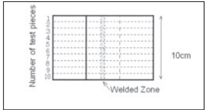
Fig. 5 — Divided region of the welded sample for shearing tensile test, optical micrograph, and SEM image observations.
