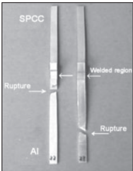
Fig. 14 — Typical rupture of Al alloy in the tensile shear strength test of SPCC/Al joints.
