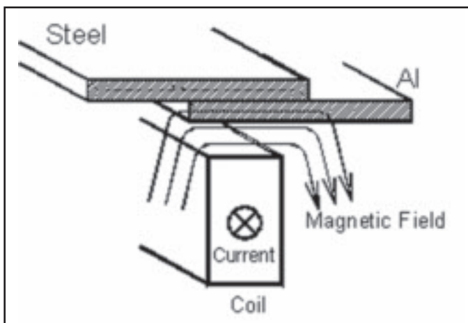
Fig. 2 — Principle of MPW for welding of the Al/steel sheet sample (cross-section view).
