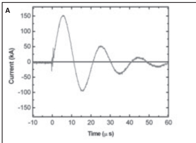
Fig. 6 — A — Typical current signal at 1.4-kJ discharge (200 µF/3.8 kV); B — bank energy vs. maximum discharge current.
