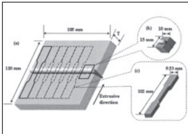
Fig. 1 — Sketch of EB-welded magnesium alloy specimen for different testing purposes.
