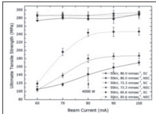
Fig. 2 — Effects of beam current and welding speed on the UTS of AZ61A weldments. Curves are linked by parameters A, E, J, O, and U with individual welding speed. Base metal UTS is 297.4 MPa.
