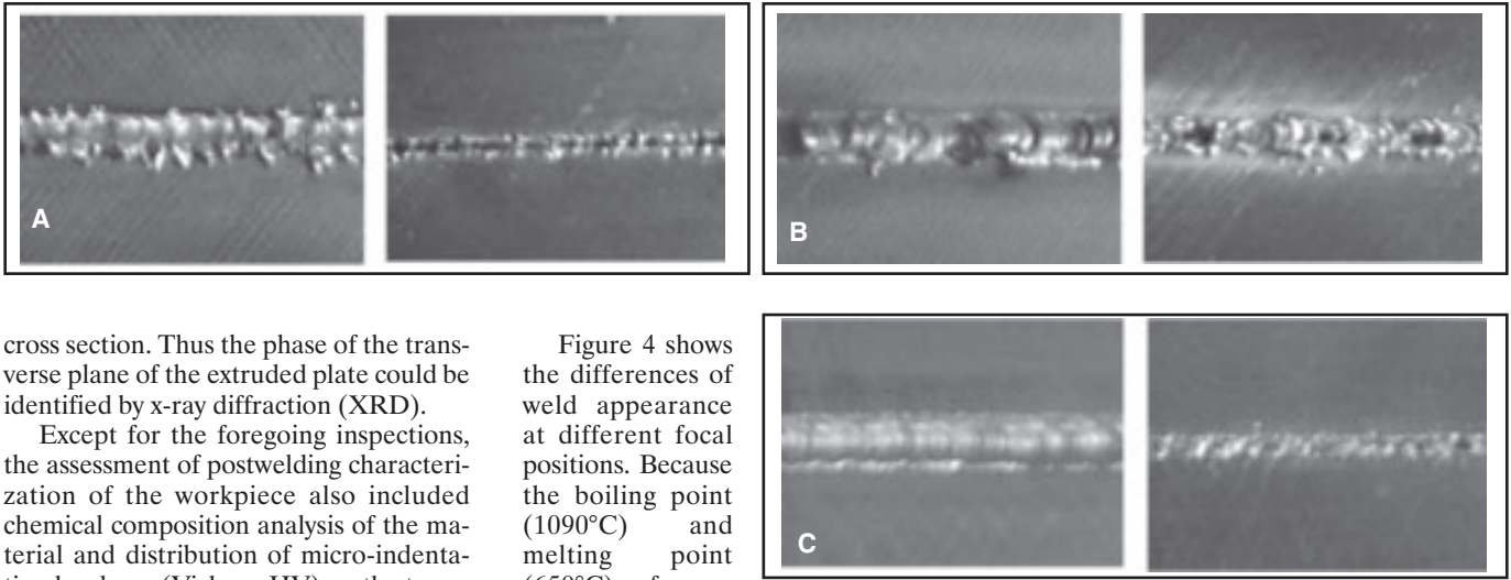
Fig. 4 — Comparison of weld appearance at different focal positions of AZ61A-F plates. Fixed conditions are 100 mA, 50 kV, and 60.6 mm/s. A — Focus at surface; B — Focus at middle; C — Focus at bottom. (crest and root respectively)
