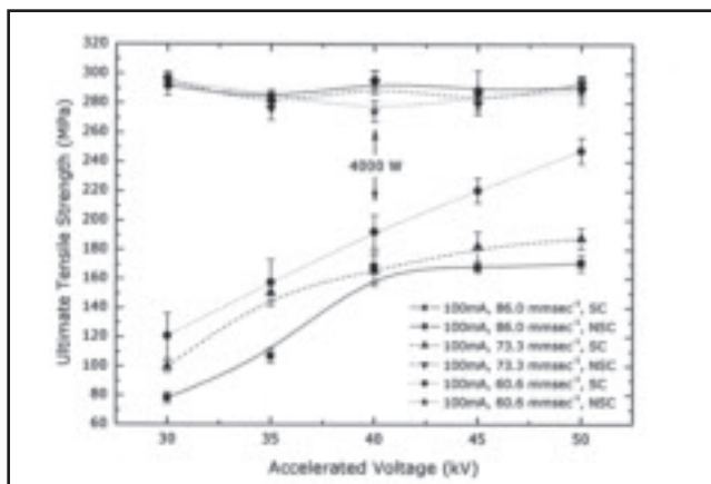
Fig. 3 — Effects of accelerated voltage and welding speed on the UTS of AZ61A weldments. Curves are linked by parameters A, F, K, Q, and W with individual welding speed. Base metal UTS is 297.4 MPa.
