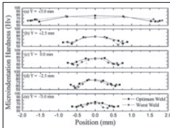
Fig. 8 — Distribution relationship of micro-indentation hardness in cross section of weld. A — Test position of microhardness; B — microhardness distribution of optimum and worst sample.
