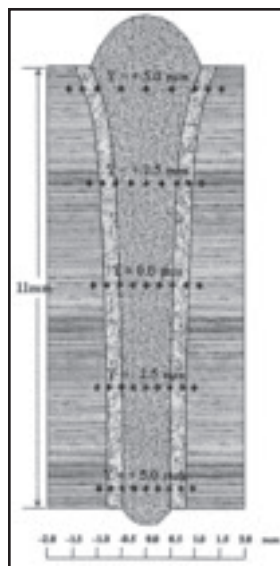
Fig. 8 — Distribution relationship of micro-indentation hardness in cross section of weld. A — Test position of microhardness; B — microhardness distribution of optimum and worst sample.
