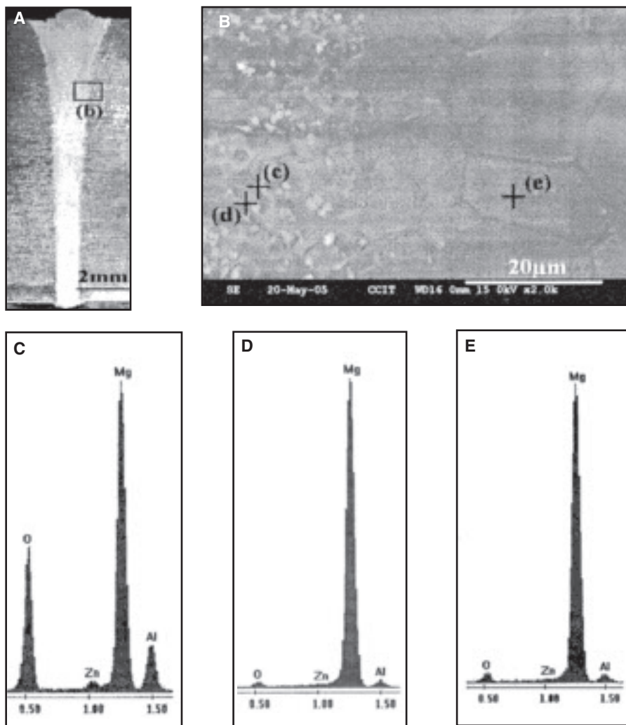
Fig. 5 — Microstructure observation and EDS analysis for the cross section of optimum weld. A — Cross section; B — SEM photograph at the weld boundary; EDS analysis. C — Particle; D — particle vicinity; E — base metal.
