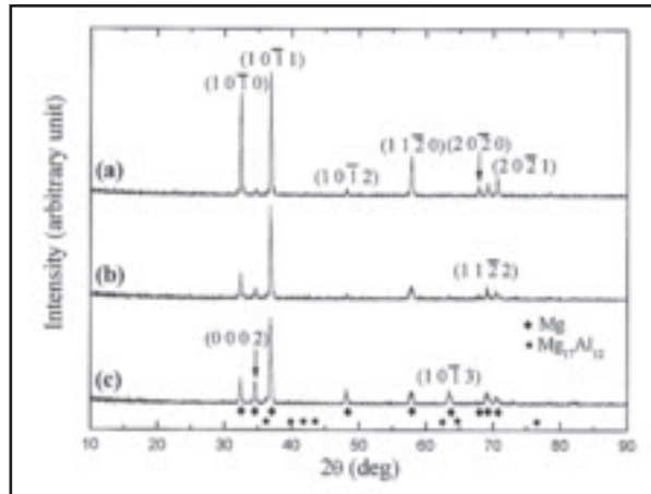
Fig. 7 — Comparison of XRD spectrum for prewelding and postwelding samples of AZ61A-F. A — Prewelding sample; B — optimum weld sample; C — worst weld sample.
