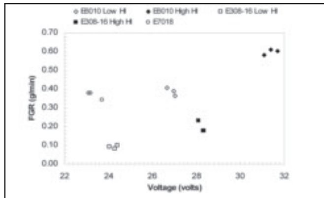
Fig. 2 — Effect of voltage on fume generation rates of E6010, E308-16, and E7018.
