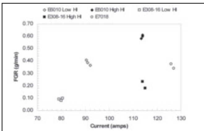
Fig. 3 — Effect of current on fume generation rates of E6010, E308-16, and E7018.
