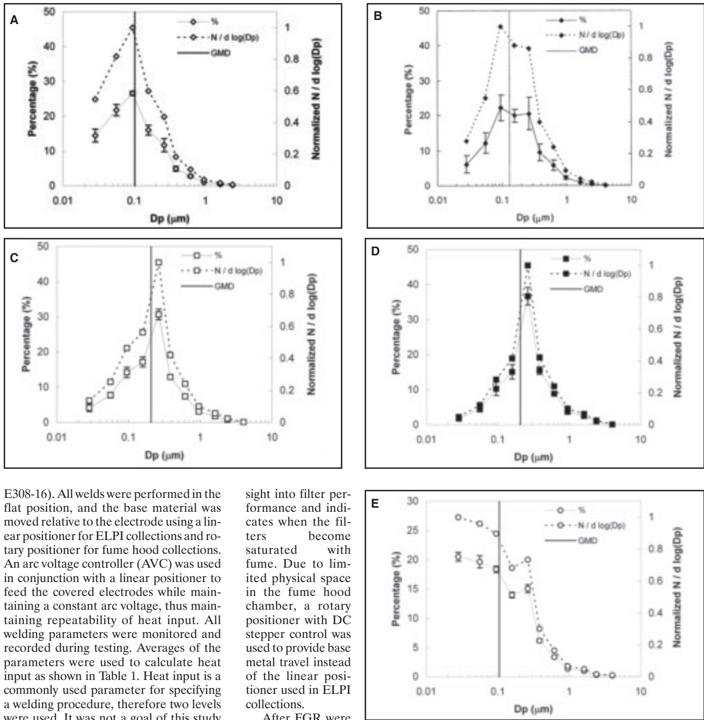
Fig. 7 — Particle number distributions as a function of particle diameter for the following: A — E6010 low heat input; B — E6010 high heat input; C — E308-16 low heat input; D — E308-16 high heat input; E — E7018 nominal heat input. Vertical lines correspond to geometric mean diameter (GMD) of distributions.
