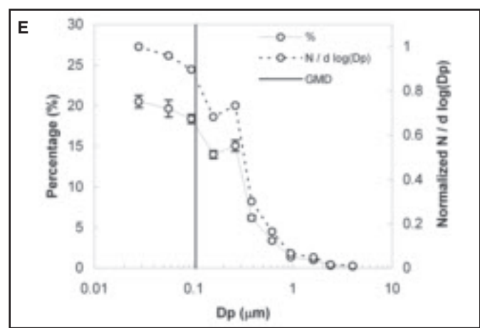
Fig. 7 — Particle number distributions as a function of particle diameter for the following: A — E6010 low heat input; B — E6010 high heat input; C — E308-16 low heat input; D — E308-16 high heat input; E — E7018 nominal heat input. Vertical lines correspond to geometric mean diameter (GMD) of distributions.
