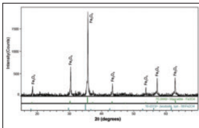
Fig. 4 — X-ray diffraction spectrum obtained from E6010 electrode (60-s collection, 16.3 kJ/in. heat input).
