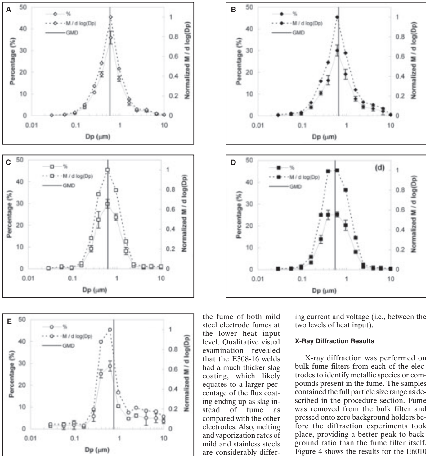
Fig. 8 — Particle mass distributions as a function of particle diameter for the following: A — E6010 low heat input; B — E6010 high heat input; C — E308-16 low heat input; D — E308-16 high heat input; E — E7018 nominal heat input. Vertical lines correspond to geometric mean diameter (GMD) of distributions.
