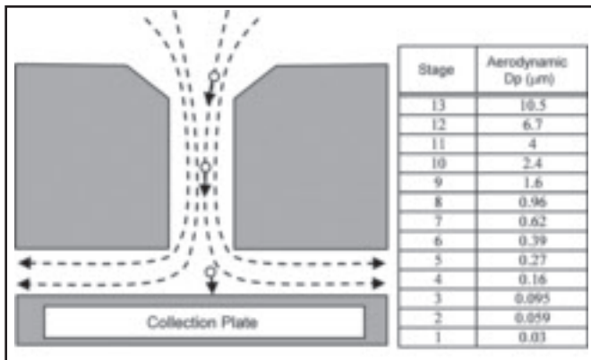
Fig. 1 — Principle of particle impaction and aerodynamic cutoff size ranges of each ELPI stage (Ref. 24).
