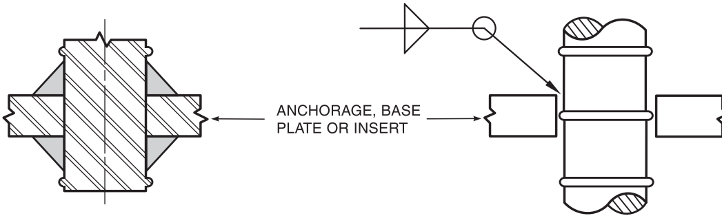
(B) EXTERNAL FILLET WELD
